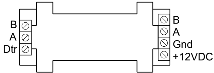
SCM-Repeater for SCM-RS2 controllers
