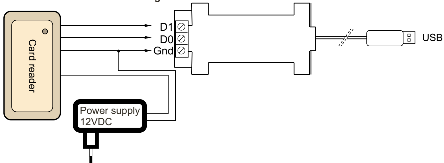
SCM-FinTerminal(AdmTerminal) - Interface for connection of card readers with wiegand 26 interface to PC USB
